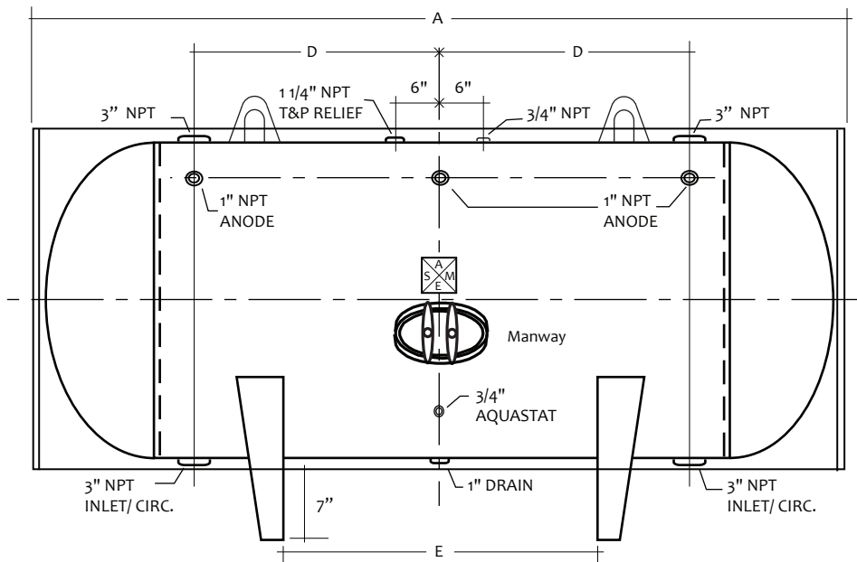
HORIZONTAL STORAGE TANK
